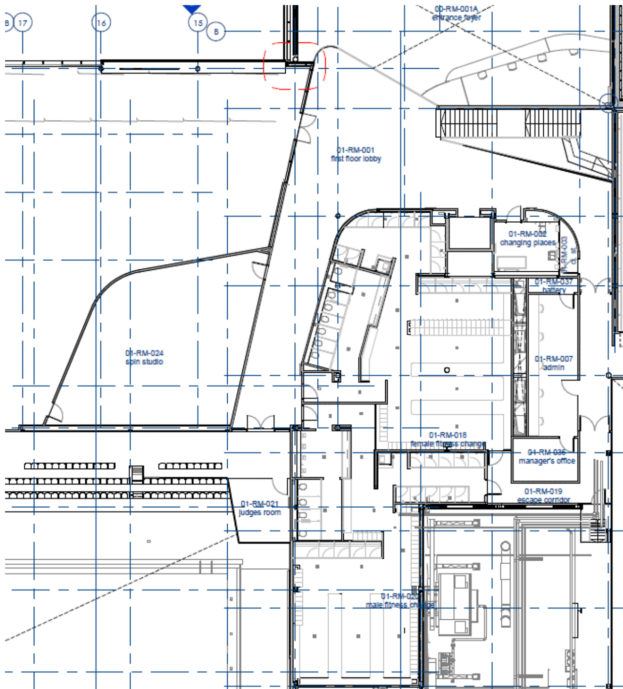
Current floor plan – WSLP first floor
